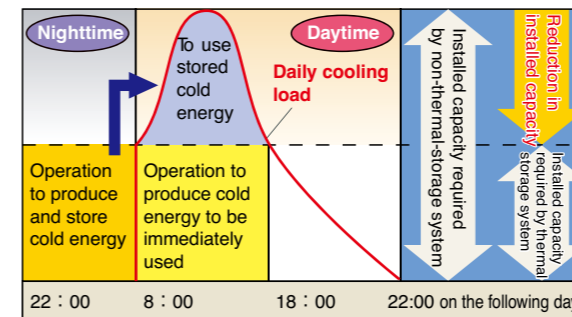
Image of Thermal Storage Operation
